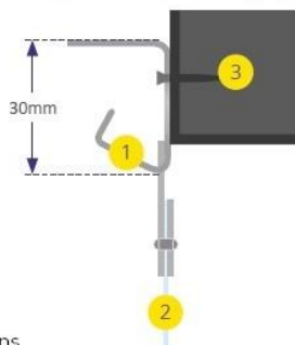
Frontal suspension
