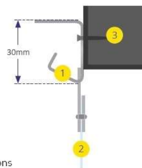
Frontal suspension
